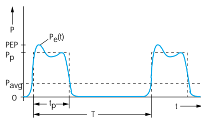
Fig. 4: Pulse power P_p (dashed line)
