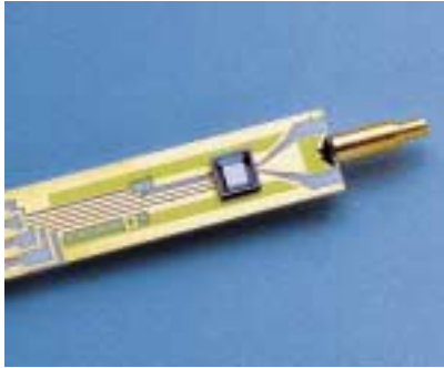
Fig. 19: Thermocouple of Power Sensors NRV-Z51 to -Z54
