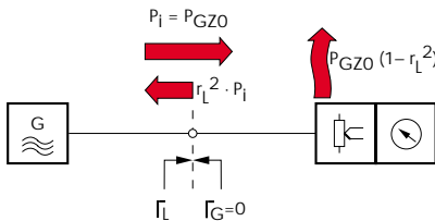
Fig. 46: Power measurement on matched source
