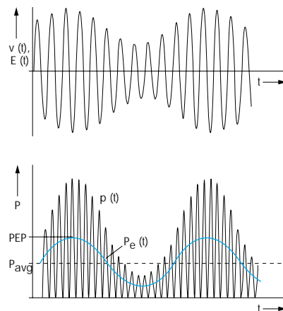
Fig. 3: Envelope of a modulated microwave signal top: voltage/field strength bottom: instantaneous power p(t) , envelope power P_e(t) , peak envelope power PEP and average power P_{avg}
