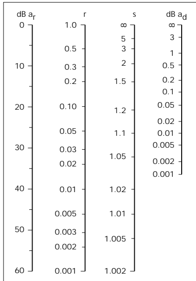
Fig. 6 Nomogram for reflection coefficient r , SWR, return loss a_r and mismatch loss a_d
