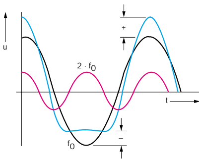
Fig. 29: Waveform distortion caused by 2nd harmonic; f_0 = fundamental frequency
