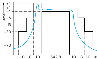
Fig. 33: GSM burst specifications and possible power envelope
